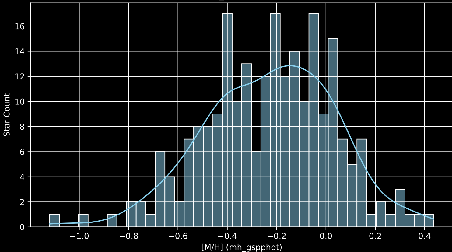
GALAH DR4 Field: [7127] [M/H] (mh_gspphot) (n= 233)
