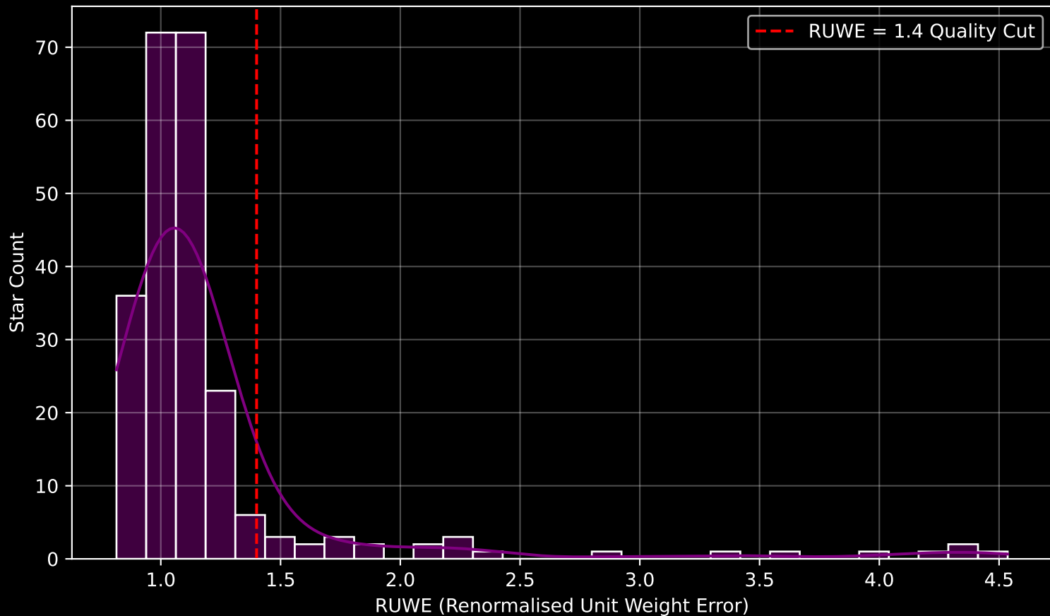
GALAH DR4 Field [7127] RUWE Distribution (n= 233)
