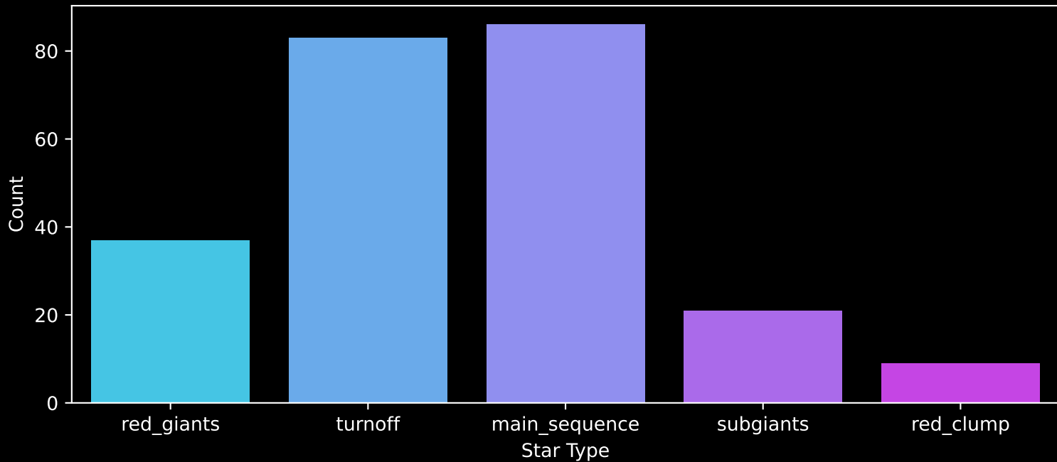
GALAH DR4 Field: [7127] Count plot of Star Type
