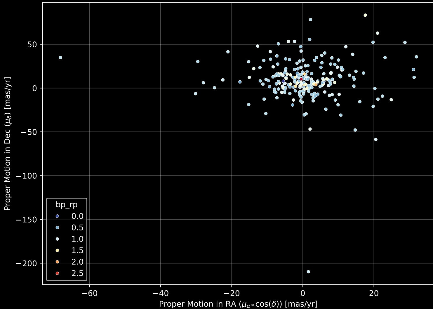
GALAH DR4 Field: [7127] Proper Motion Diagram (n= 236)
