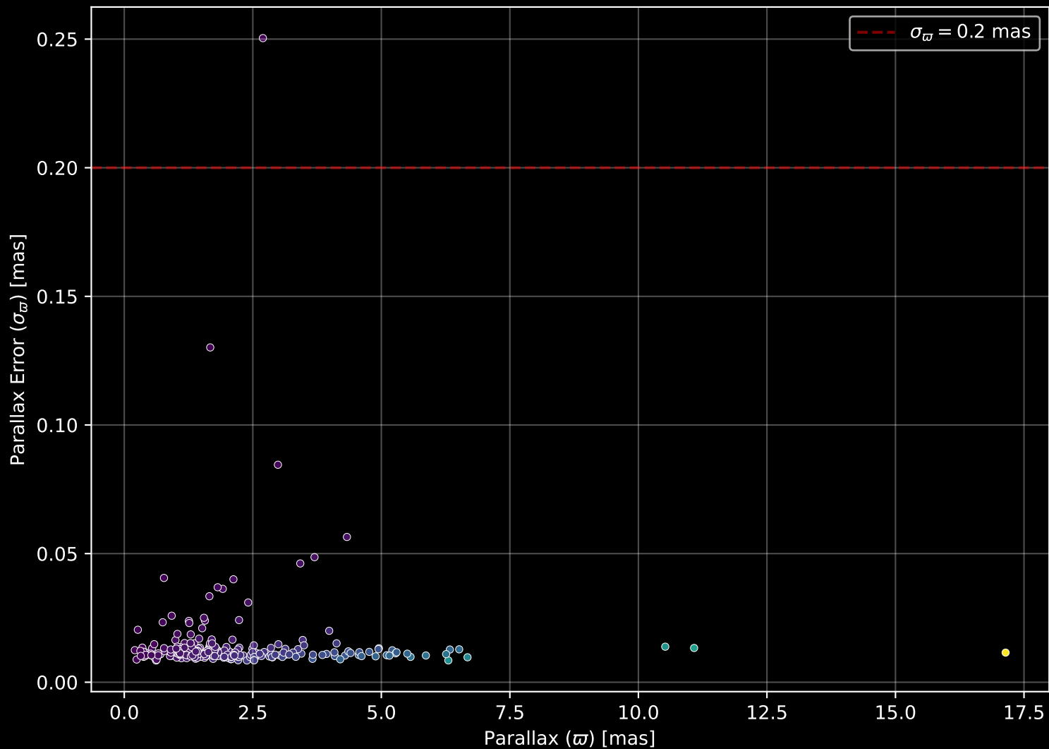
GALAH DR4 Field: [7127] Parallax Quality (n= 236)
