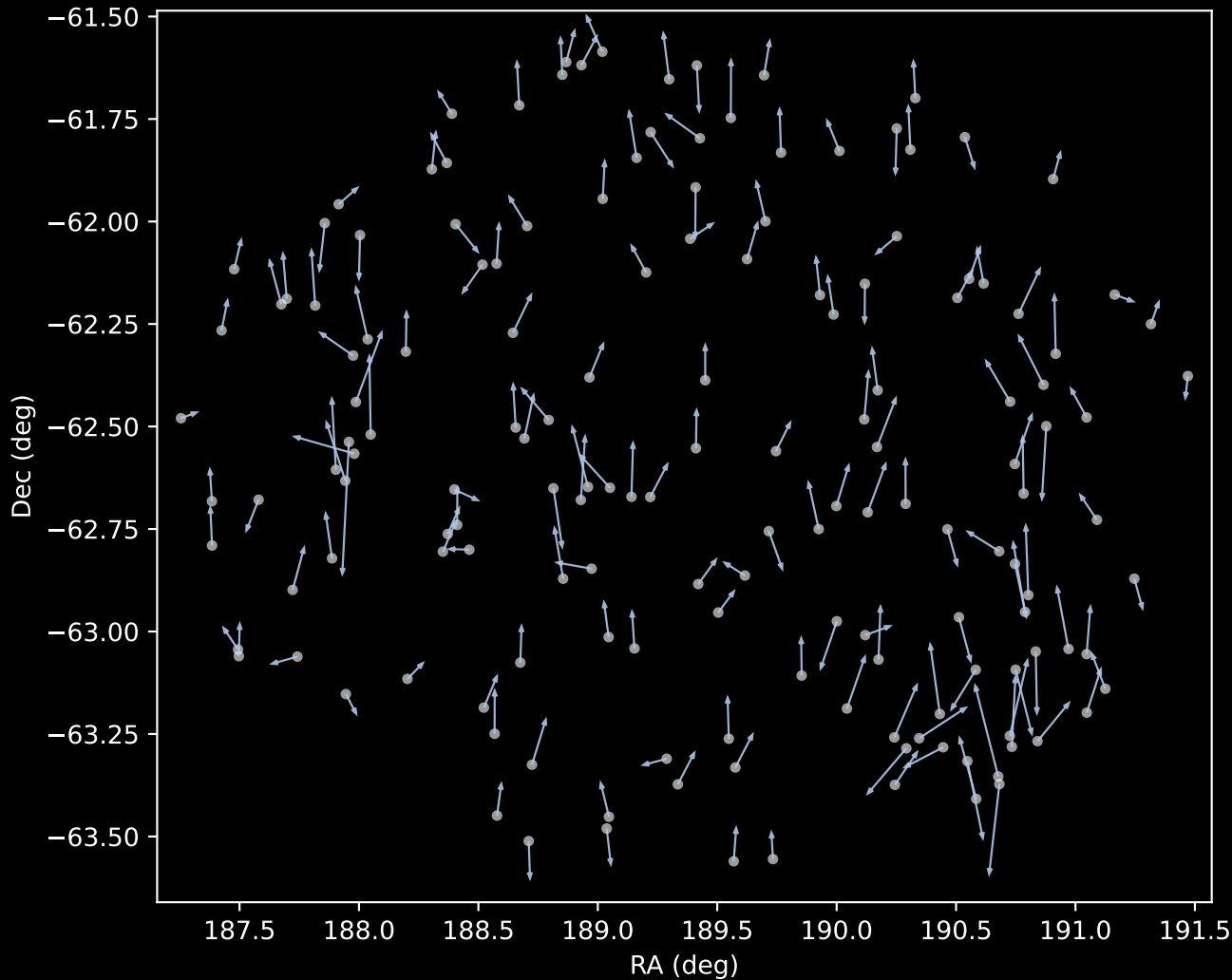
GALAH DR4 Cluster 1 Proper Motion Vectors (n=159)
